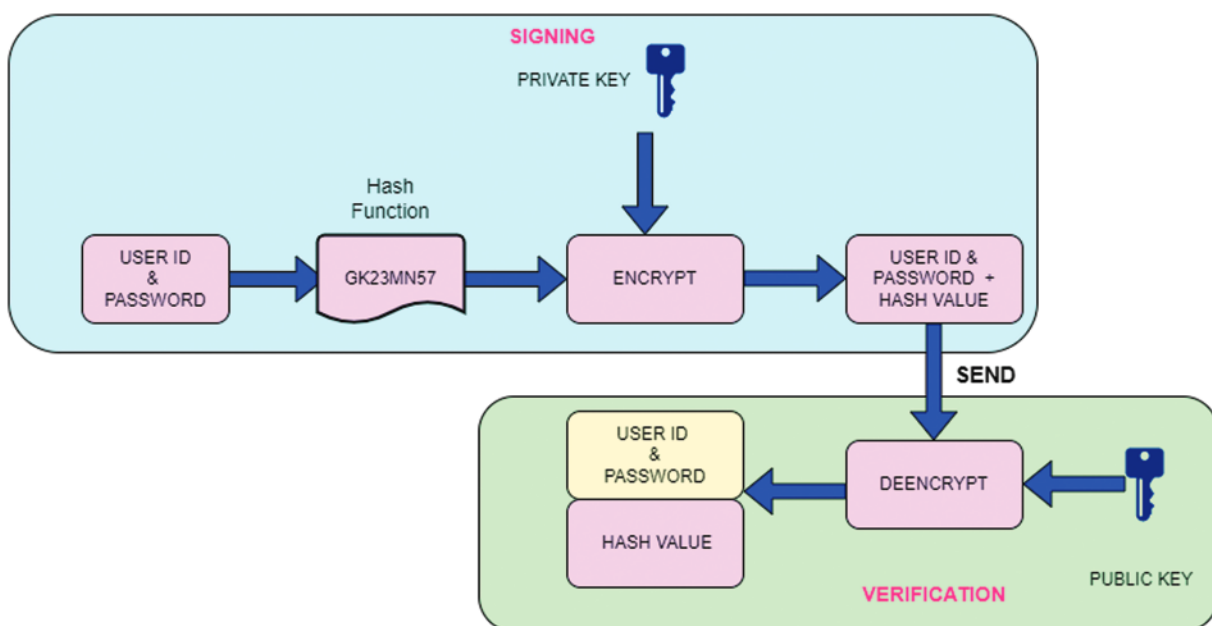
Figure 2: Workflow of the verification process
